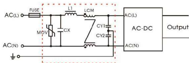
Fig 4: EMC circuit for harsh requirements
