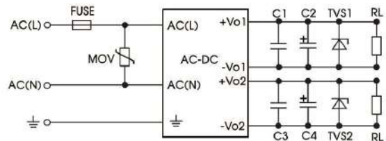
Fig. 2: Typical circuit diagram for SLHE10-20Dxx series
