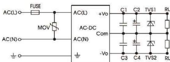
Fig. 1: Typical circuit diagram for SLHE10-20Axx series
