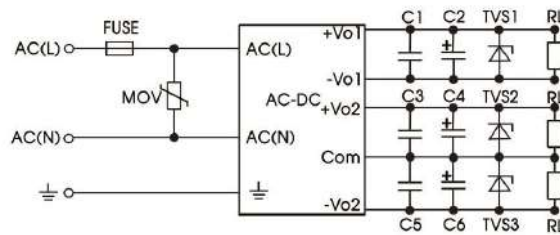
Fig. 3: Typical circuit diagram for SLHE10-20Cxx series
